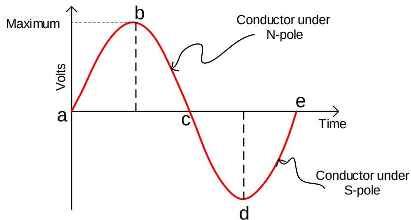
Fig 1.07. Generated emf.
